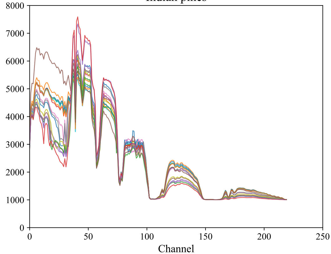
Indian pines
